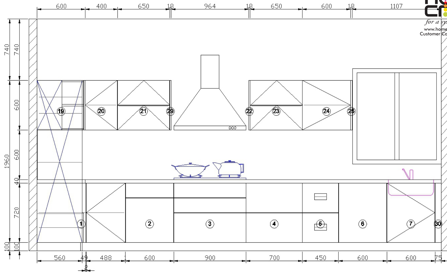
A View elevation drawing
